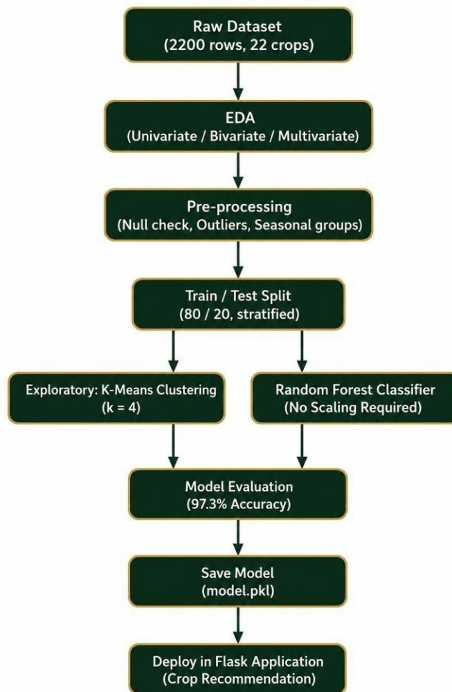
Figure 3.1: End-to-end machine learning workflow, from raw data to saved model.
