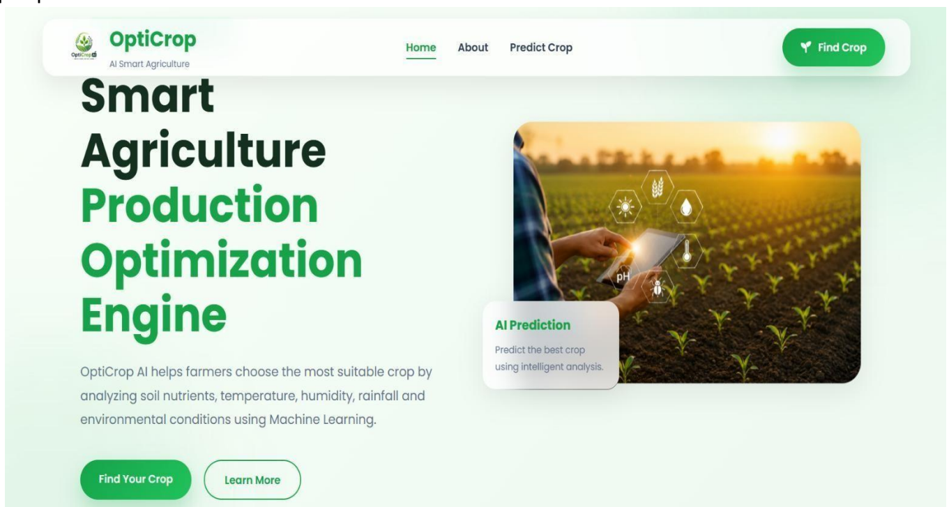
Figure 4.1: Home page.
